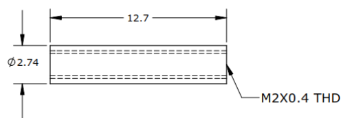
CORE
